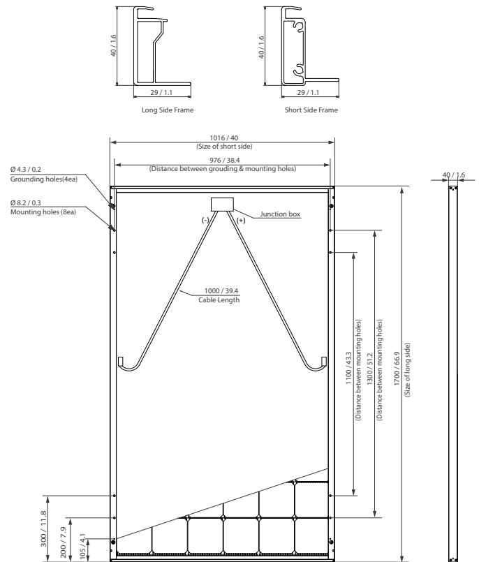
The distance between the center of the mounting/grounding holes.
